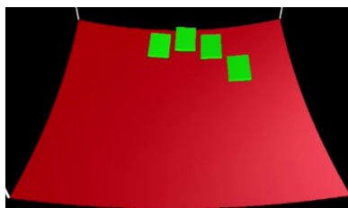
Figure 6. Curvature function.
